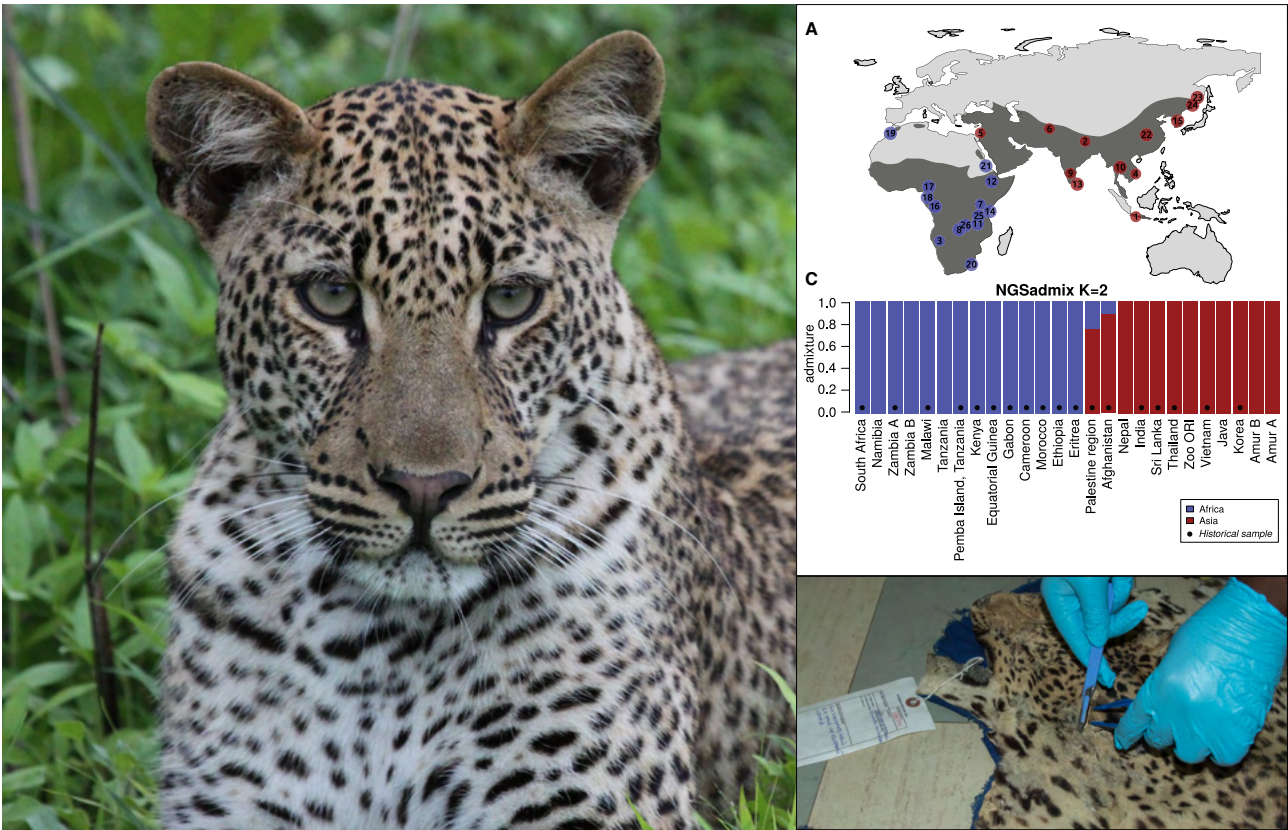
Similar to lions, new genetic tools developed from Zambian leopard work combined with genomic information on leopards rangewide (see Scientific Publications Pajmans et al. 2021) will greatly assist anti-trafficking efforts by providing intelligence and forensics information.
