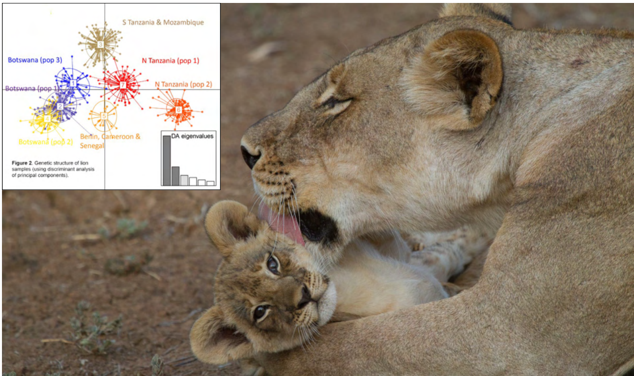
Cutting-edge genetic tools developed from long-term work on lions now provide intelligence and forensics to combat trafficking of lion skins and parts by enabling the tracing back of trafficked lions to their source populations. Inset: Baseline genetic data from lions across Africa demonstrate clear distinctions across regions and populations.
